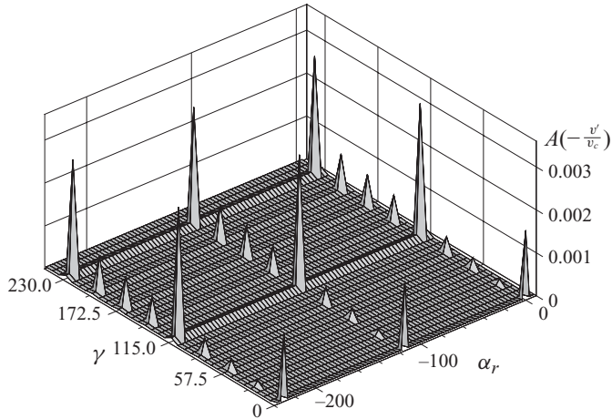
FIGURE 12. A discrete Fourier amplitude spectrum for the non-dimensionalized disturbance velocity v'/v_c over the streamwise ( \alpha_r )–spanwise ( \gamma ) wavenumber plane for hole array that is finite in the x -direction.
