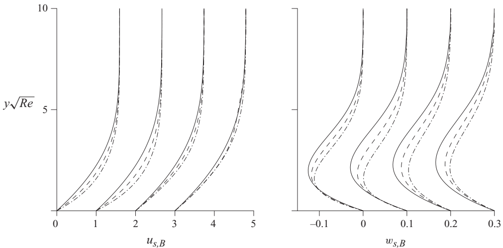
FIGURE 16. Streamwise and CF velocity profiles in a streamline coordinate system of base flow (————) and mean flow (base flow + mode (0,0)) for the Homog-low (-----) and Homog-high (-·-·-·-) cases, at different streamwise positions ( x = 4, 5, 6, 7 from left to right). The abscissa is successively shifted by 1 and 0.1, respectively.
